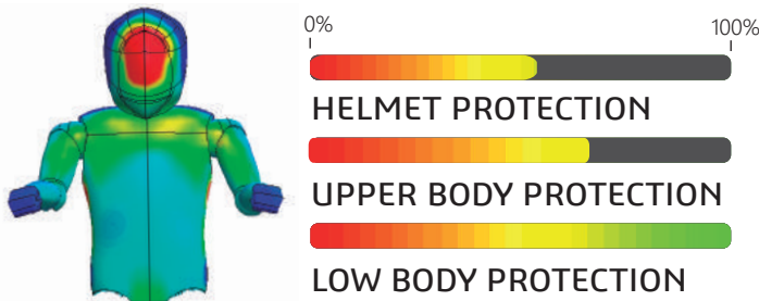
WITHOUT DEFLECTOR
